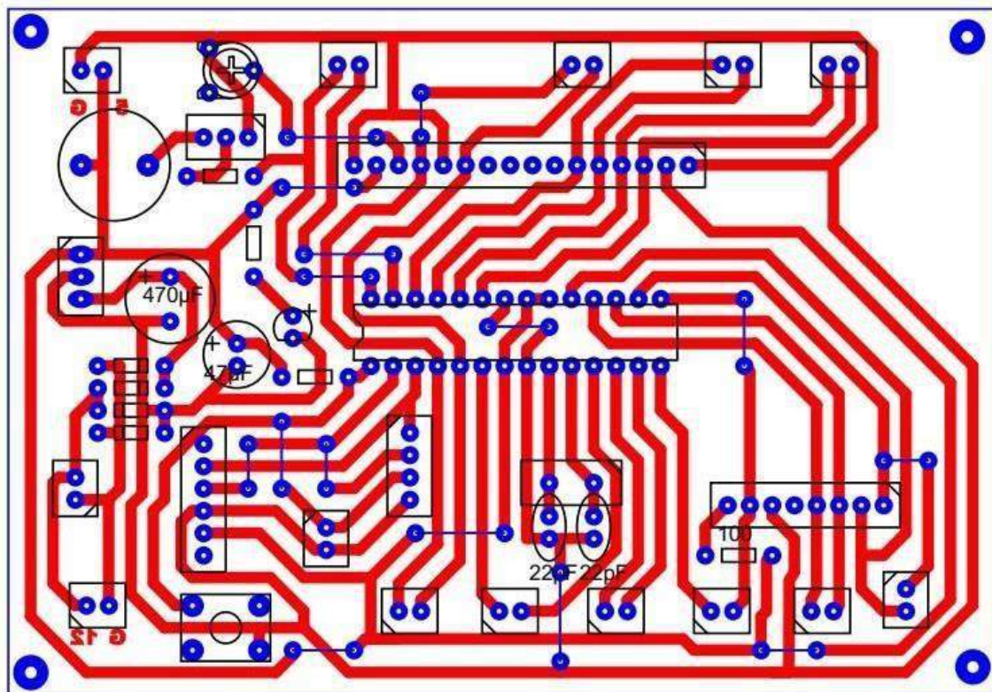
Fig 25 PCB design
